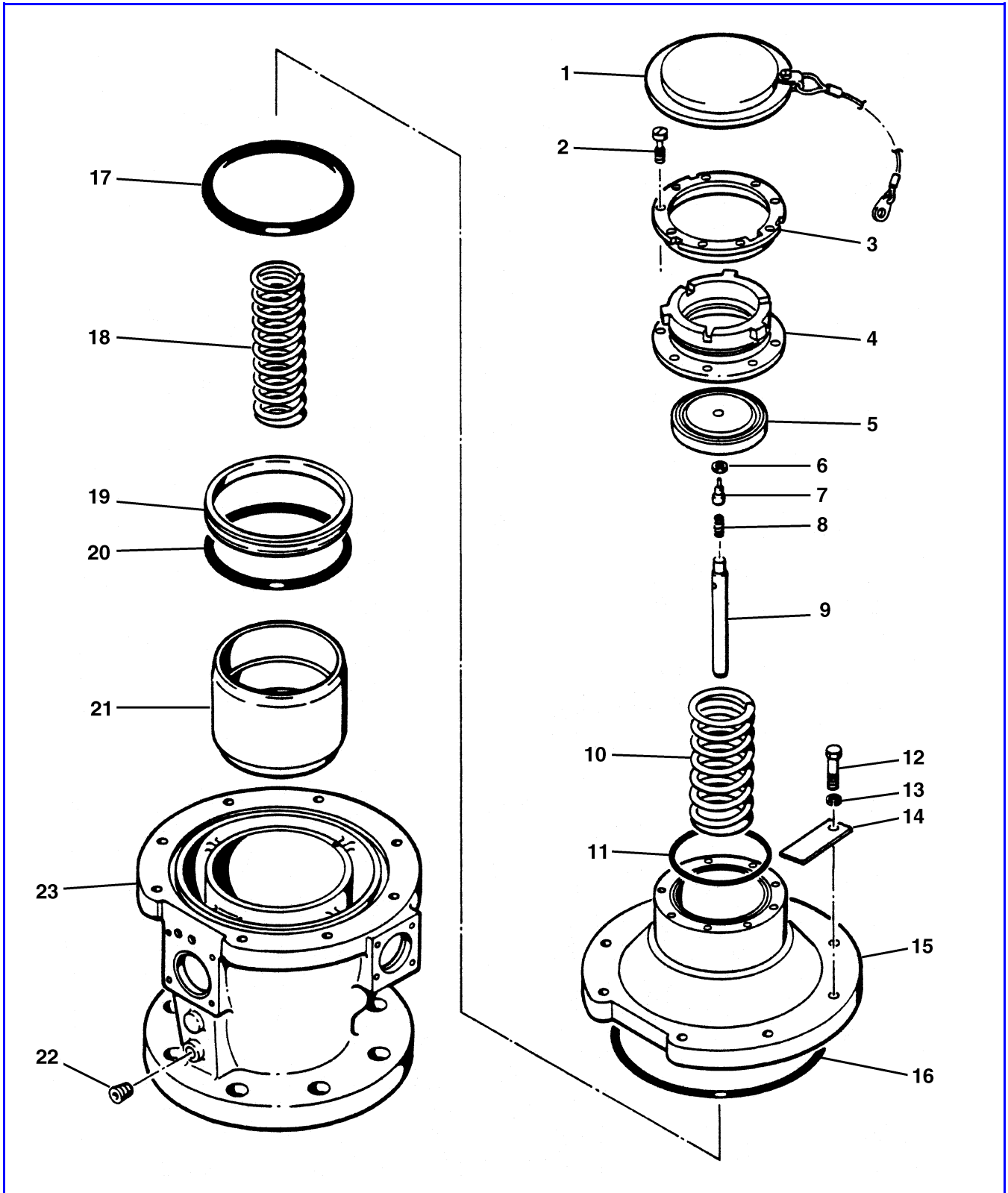
IPL Figure 2. 4-Inch by 2½-Inch Hydrant Valve Body and Piston Assembly
