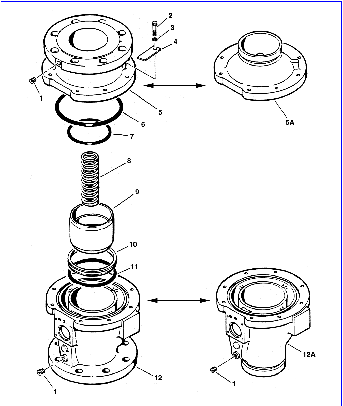
IPL Figure 1. 4-Inch In-Line Control Valve Body and Piston Assembly
