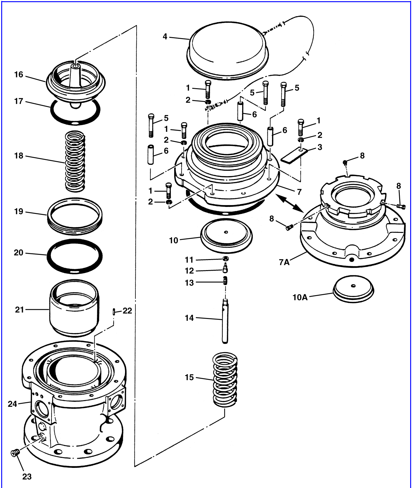
IPL Figure 3. 4-Inch by 4-Inch Hydrant Valve Body and Piston Assembly
